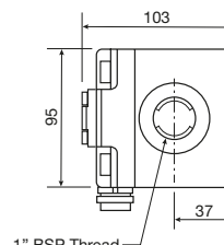
316 St St body
